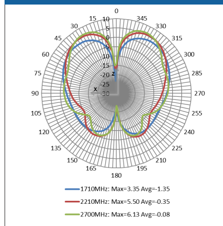
Side to Side XZ at 1710-2700MHz
