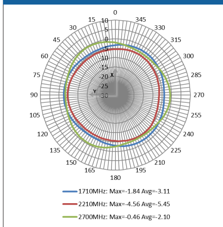
Azimuth XY at 1710-2700MHz
