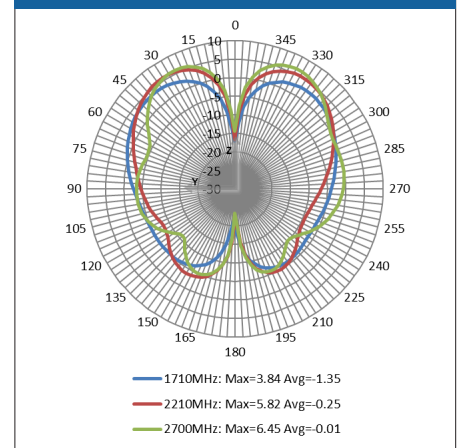
Front to Back YZ at 1710-2700MHz
