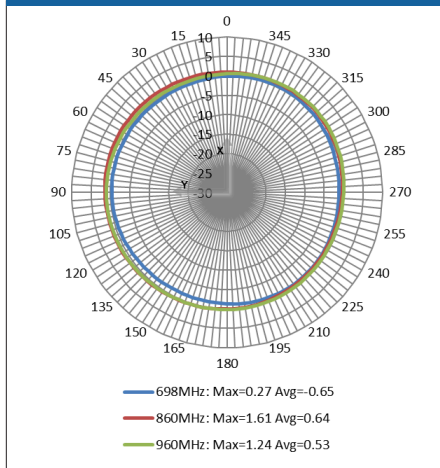
Azimuth XY at 698-960MHz
