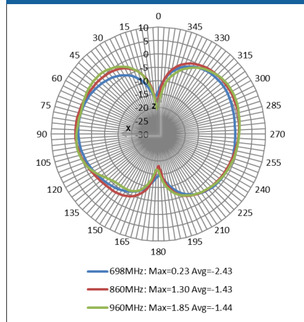
Side to Side XZ at 698-960MHz
